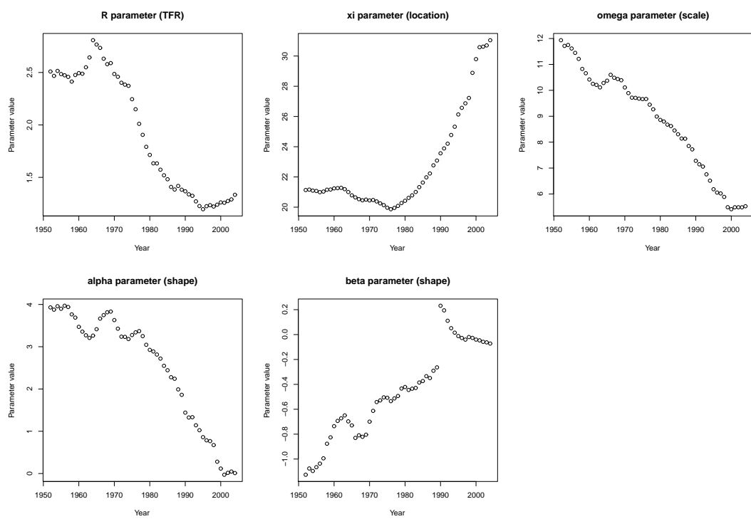
Figure 7: Trends of parameters estimated from the FGSN model. Italy (1952-2003)
