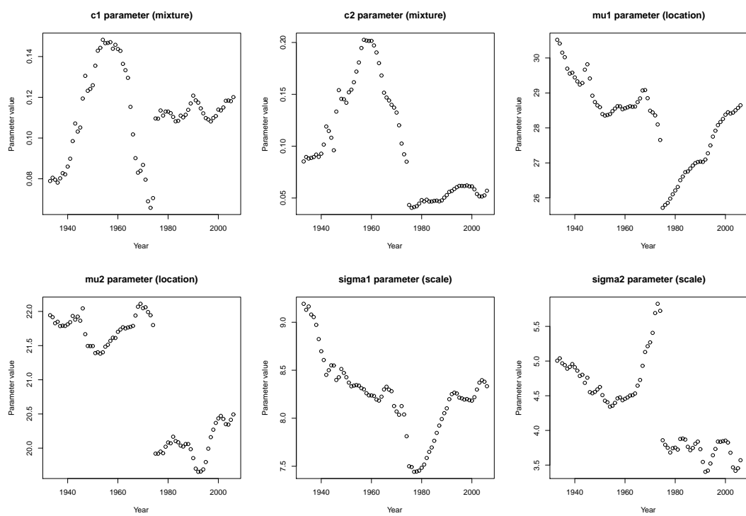
Figure 11: Trends of parameters estimated from the Peristera-Kostaki mixture model. USA (1933-2006)
