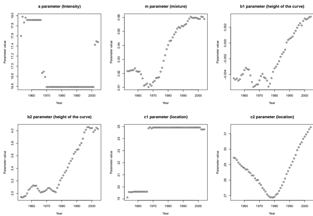
Figure 9: Trends of parameters estimated from the Hadwiger mixture model. Italy (1952-2003)
