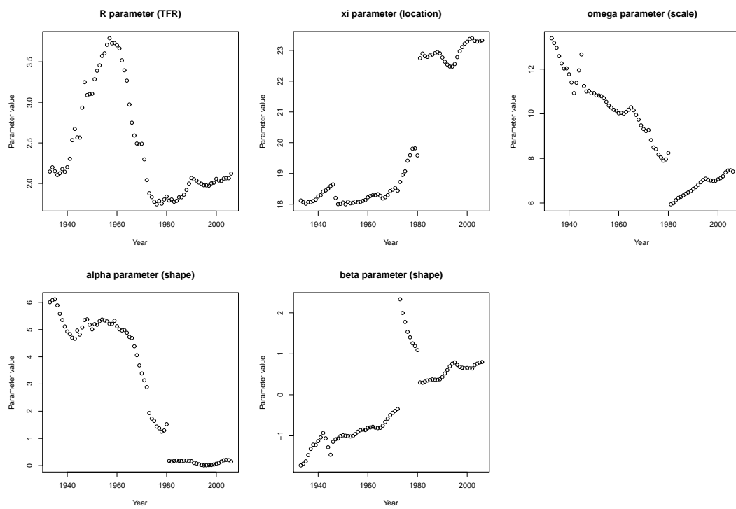
Figure 10: Trends of parameters estimated from the FGSN model. USA (1933-2006)
